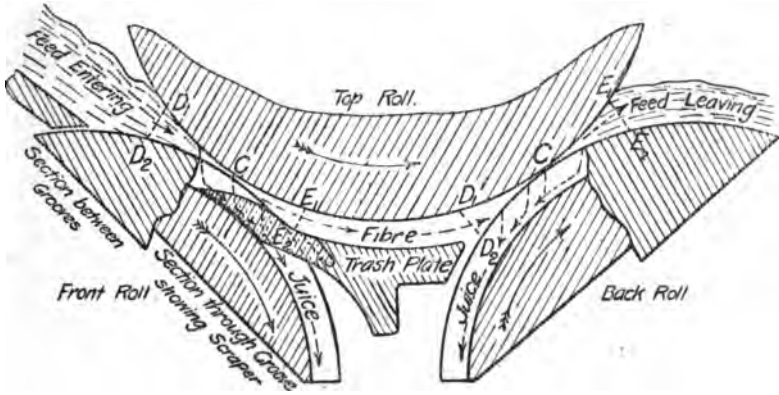
FIG. 10.—MESSCHAERT GROOVING OF ROLLERS (Vertical Section)
